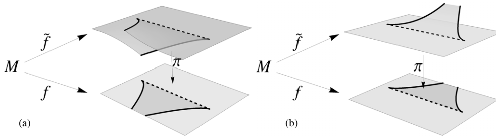
Figure 3. Two examples of unfoldings of bifurcation diagrams. The two unfolded momentum domain pictured are what we call (a) pleat and (b) flap. Thick lines (both solid and dashed) represent critical values. Solid thick lines represent the image of elliptic singularities while dashed thick lines represent the image of hyperbolic singularities.
