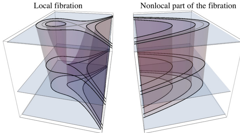
Figure 5. A Poincaré surface of a section for the vector field X_1 with level sets of the function f_1 (horizontal planes) and the function f_2 . The fibres of f that contain this set are topologically compact. This fact is pictorially represented by adding the intervals that connect endpoints of the same component. The section in this picture is cross-multiplied with S^1 . The subset associated to f_1 > 0 is that whose vertical component is above the singular point. The lighter figure-of-eight curve corresponds to a bitorus.
