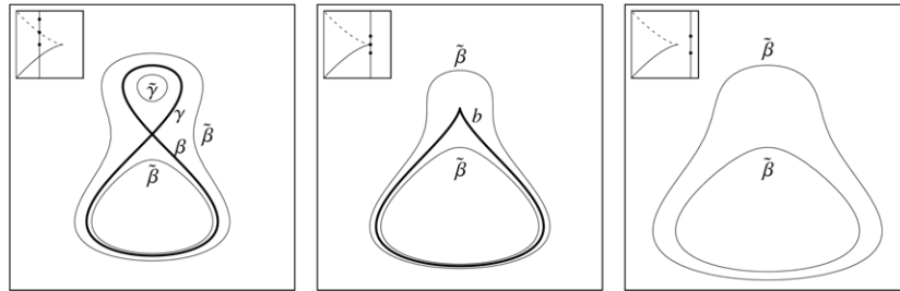
Figure 6. Homology cycles for fibres in a neighbourhood of a cusp singularity. Here the intersections of fibres with the Poincaré surface of section \Sigma are shown and the homology cycles supported by these intersections are marked. Singular level sets (bitorus, cuspidal torus) are drawn with thicker lines. For each fibre the corresponding projection to the base space of the fibration is shown. Note that in the leftmost panel, the two components denoted by \tilde{\beta} and \tilde{\gamma} inside the bitorus project under f to the same point in the interior of the cusp, although they project under \tilde{f} to different points in the unfolded momentum domain: \tilde{\gamma} projects under \tilde{f} inside the flap while \tilde{\beta} projects outside the flap, see figure 2.
