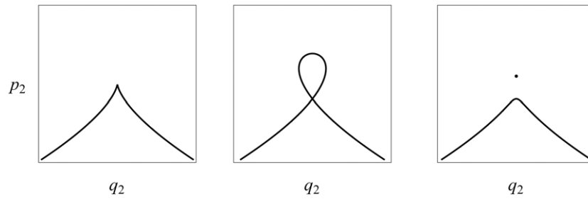
Figure 4. From left to right: intersections of the cuspidal torus, the bitorus and the disjoint union of a torus and a circle with the p_1 = 0 plane in a neighbourhood of the cusp singular point to form respectively a cuspidal set, a bitoric set and an elliptic set, see figure 5, left panel. In the elliptic case the critical points lie on an isolated line that intersects the p_1 -plane in a point.
