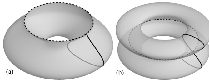
Figure 1. Singular fibres: (a) cuspidal torus and (b) bitorus. The dashed lines represent the singularities of the fibres. These singularities are critical points of f .
