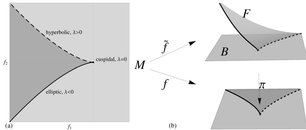
Figure 2. (a) The local bifurcation diagram of a cusp singularity and (b) its associated unfolded momentum domain. The two-component region is represented by the darker gray shade.
